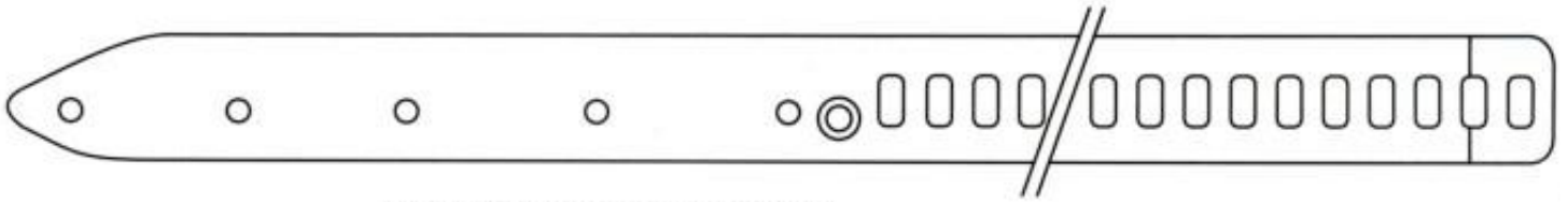
IMAMURA RAPIER TAPE SR107
