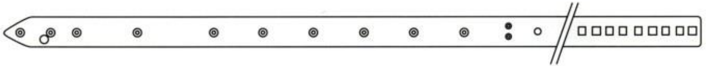
ISHIKAWA RAPIER TAPE 1001 FOR NYLON SUPPORT WIDTH 24 mm. LEFT
