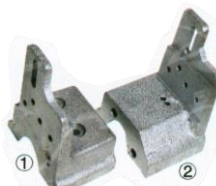
TEMPLE SEAT, CODE: PNM71986, PNM71985
